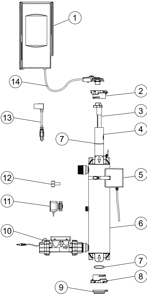
Figure 1 System Components
